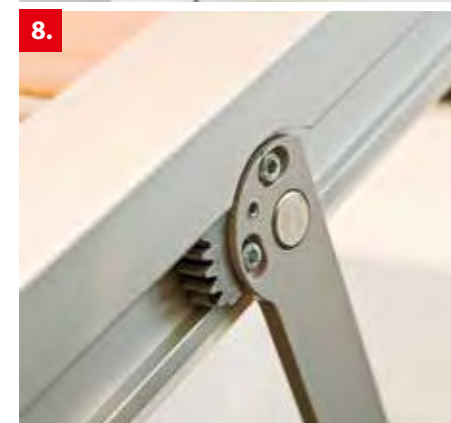
FOTO 8: Staffa per mensola basculante. PHOTO 8: Jointed arm for tilting shelf.
